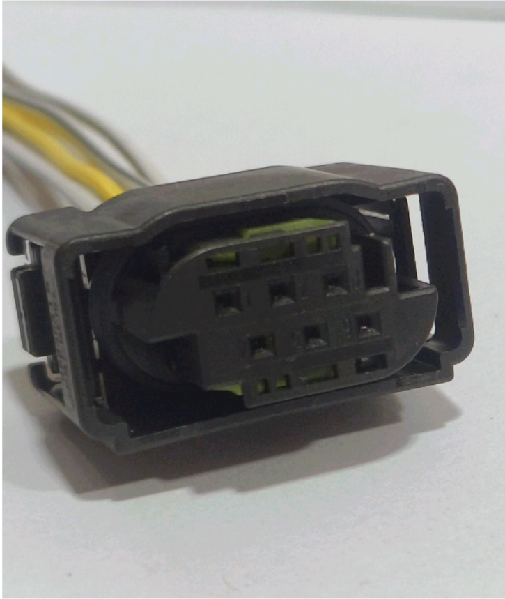
Throttle Body Cng coupler
