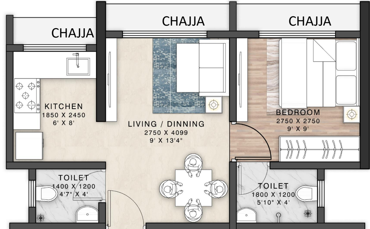
TYPICAL UNIT PLAN B
