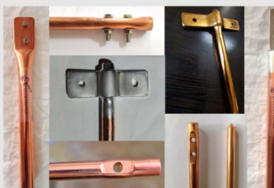
COPPER LUGS
